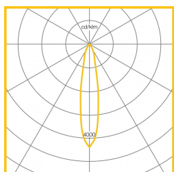
4000K 1683 lm 22W Narrow LOR = 100%
