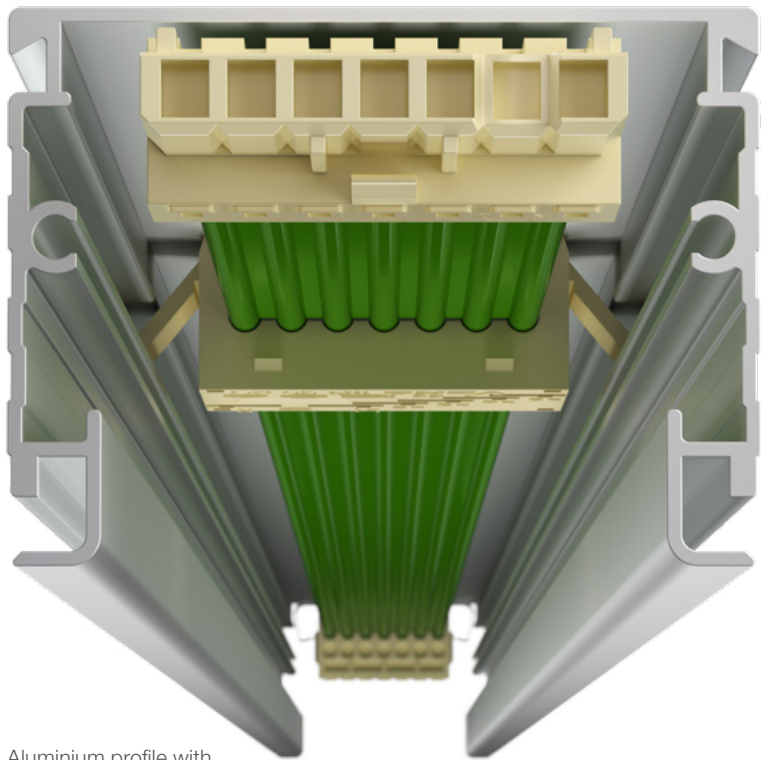
Aluminium profile with 7, 10 or 13 cores.
