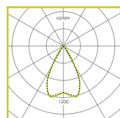
Flood 54° 9W LED 500 lumens 4000K • LOR = 100%
