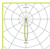
Spot 24° 9W LED 500 lumens 4000K • LOR = 100%
