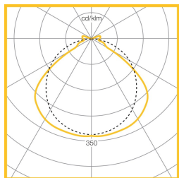
Symmetric Wide 42W LED 5006 Lumens LOR = 100.0% SHR MAX = 1.83
