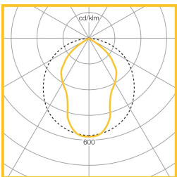
High Rack 79W LED 10296 Lumens LOR = 100.0% SHR MAX = 1.06
