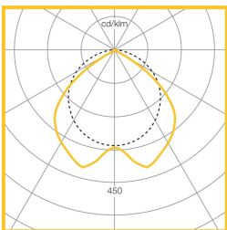
Symmetric Medium 21W LED 2508 Lumens LOR = 100.0% SHR MAX = 1.91
