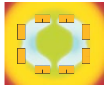
Typical Theatre lighting levels utilising DTFN Elite.
