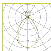
70W LED Micro Prism • LOR = 100% • SHR MAX = 1.45
