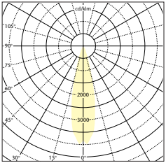
Low Voltage IP65 Downlighter LDR 9102 - IP65 50W LV Capsule Lamp
