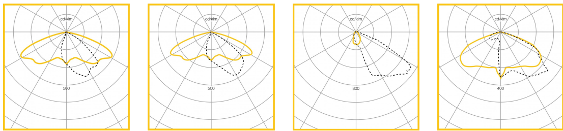
Road Optic | 19,840 lumen | 170W LOR = 100%
