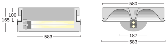
Single lamp
