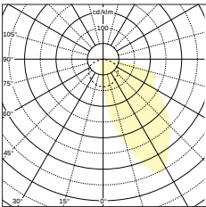
Asymmetric Wallwasher 1 x 55W TC-L Compact Fluorescent Lamp
