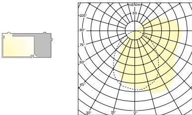
Cornice LINEAR SURFACE 1 x 1200mm PRISMATIC DIFFUSER 36W Lamp
