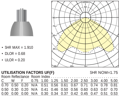
Atlanta 4 X 42W TC-T Lamps 400mm Ø Acrylic Reflector
