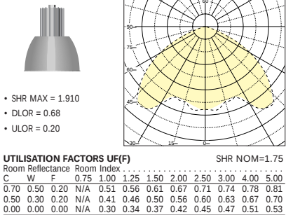
Atlanta 4 X 42W TC-T Lamps 400mm Ø Acrylic Reflector
