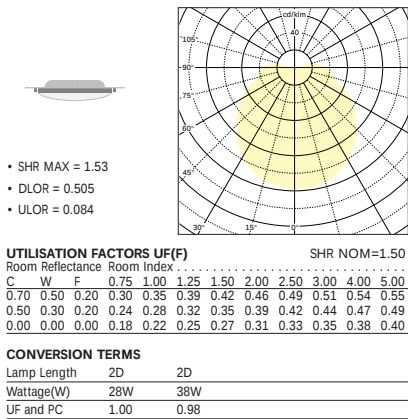
Laguna 1 x 28W 2D COMPACT FLUORESCENT
