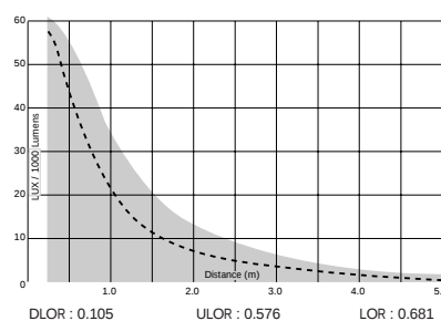
Flight Wall Mounted 2 x 55W TC-L Compact Fluorescent
