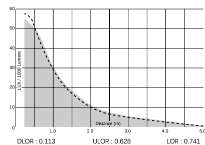
Flight Free Standing 4 x 55W TC-L Compact Fluorescent
