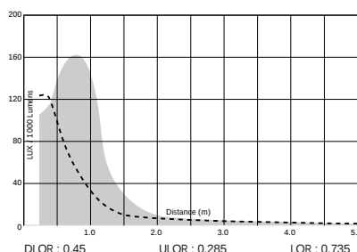
Oasis® Asymmetric Wall Mounted 1 x 55W TC-L Compact Fluorescent
