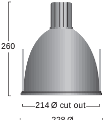
Spectre 200 35W/70W/150W CDM-T
