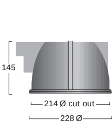
Spectre 200 2 x 18W TC-D
