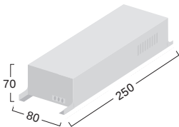
35W CDM-TC Gearbox supplied complete
