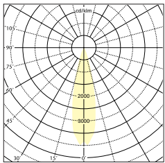
Low Voltage IP65 Downlighter LDR 1002 - IP65 20W LV Capsule Lamp
