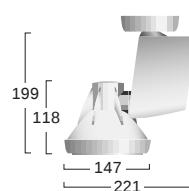
TNS-T 75-100W LV Tungsten Halogen Integral transformer
