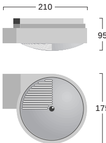
Pre-wired power feed DT-LPFO5-1053
