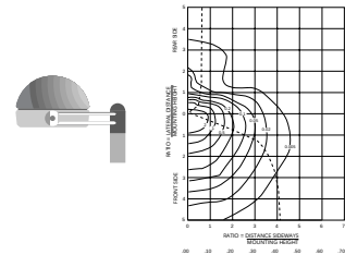
Magnudisc 150W SON Distribution T - Forward Throw
