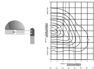
Magnudisc 150W SON Distribution P - General Area
