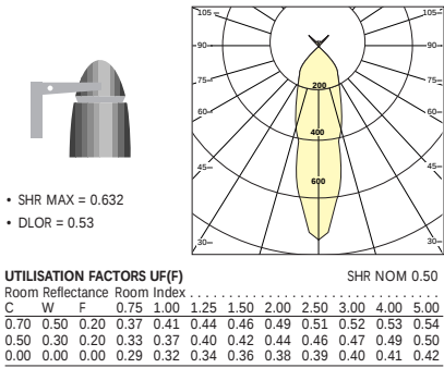
Ergo Large 1 x 70W CDM-T Lamp
