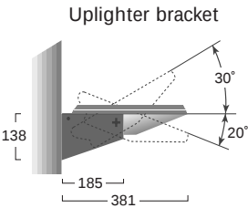
Uplighter bracket
