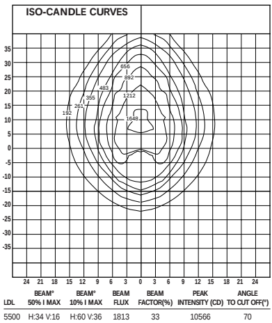
Microliter 70W SON WIDE
