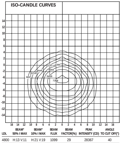
Microliter 70W HQI NARROW
