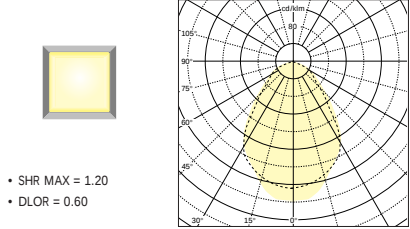
Canopy Master CM60 250W SPECULAR REFLECTOR AND PYRAMID LENS 250W HQI-T
