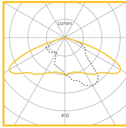
Symmetric Wide Beam 150W 15165 Lumen LOR = 100.0%
