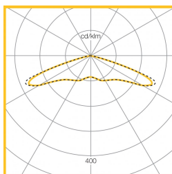
Symmetrical Square Beam 68W 6355 Lumen LOR = 100.0%
