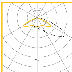
Area Optic 60W 7669 Lumen LOR = 100.0%
