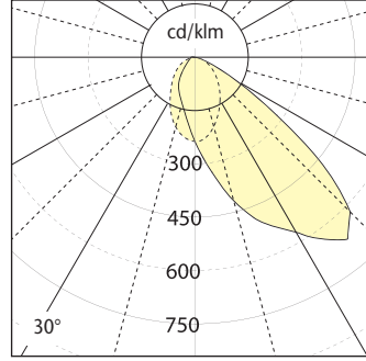
1 x 150W CDM-TD Lamp SPF150P
