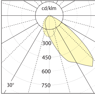
1 x 70W CDM-TD Lamp SPF70P
