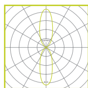
Direct/indirect 45W LED 3527 lumens, 4000K • LOR = 100%
