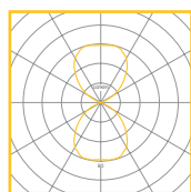
Direct/indirect 2 x 26W TC-T 3000K • LOR = 36%
