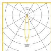
Direct 1 x 70W CDM-T 3000K • LOR = 59.8%
