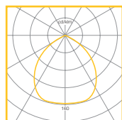
Direct 1 x 26W TC-T 3000K • LOR = 36%
