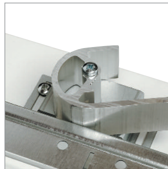
Cam jacking bracket modular ceilings
